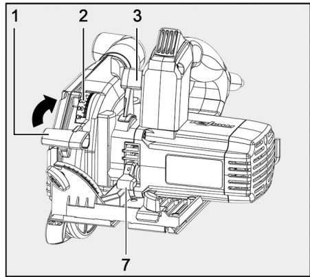
Fig. 12: Plunge cutting
