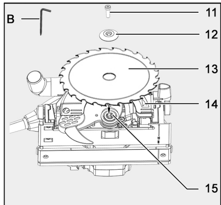
Fig. 5: Replacing the saw blade
