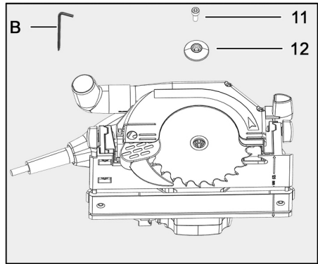
Fig. 4: Removing the old saw blade
