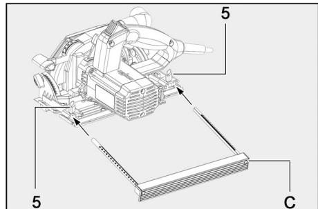
Fig. 17: Installing the parallel guide fence
