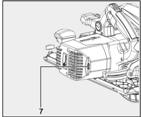
Fig. 15: Selecting the rotational speed at the setting wheel
