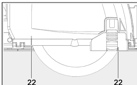
Fig. 18: Plunge cutting
