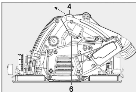
Fig. 10: Switching the machine on
