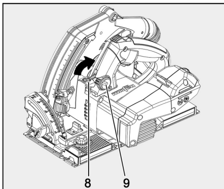
Fig. 5: Unlocking the guard cover
