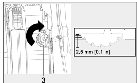
Fig. 24: Activating the pre-scoring function
