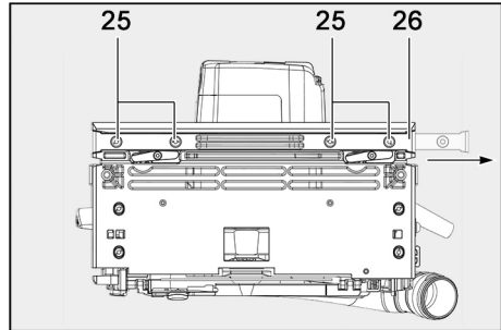
Fig. 23: Removing the insert for third-party rail
