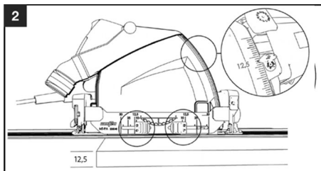
Fig. 27: Setting the cutting depth
