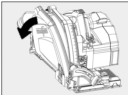
Fig. 6: Opening the guard cover
