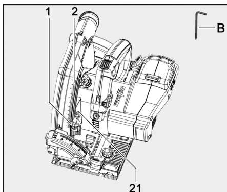
Fig. 14: Setting the cutting depth
