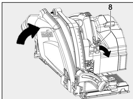
Fig. 9: Closing the guard cover
