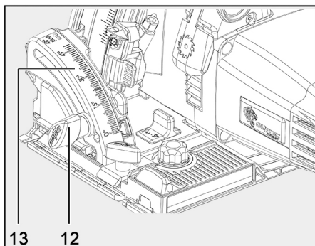
Fig. 15: Setting the saw unit for bevel cuts
