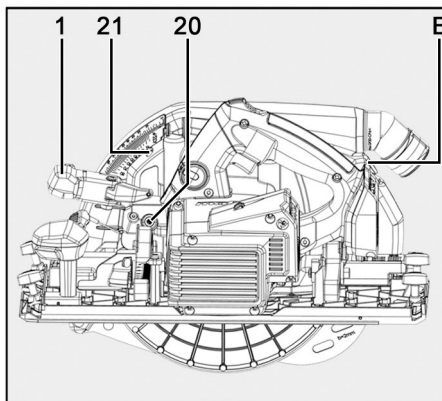
Fig. 19: Resetting the cutting depth
