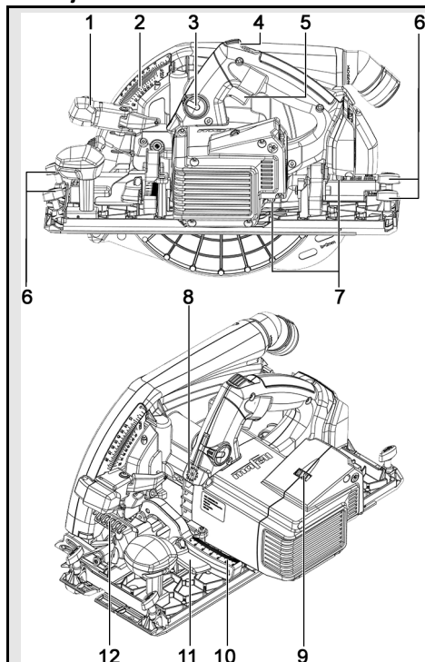
Fig. 2: Adjustment elements
