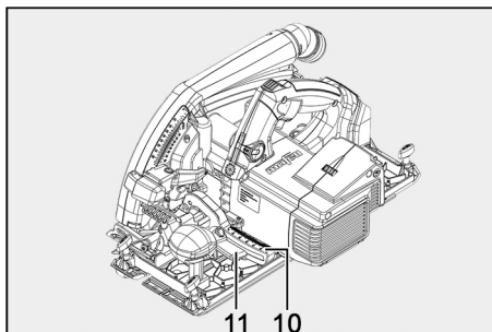
Fig. 16: Setting the saw unit for bevel cuts
