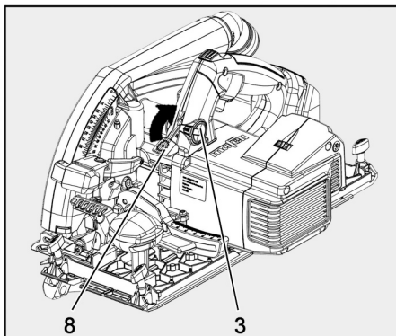
Fig. 5: Locking the saw shaft
