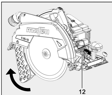
Fig. 6: Opening the guard
