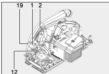
Fig. 17: Plunge cutting
