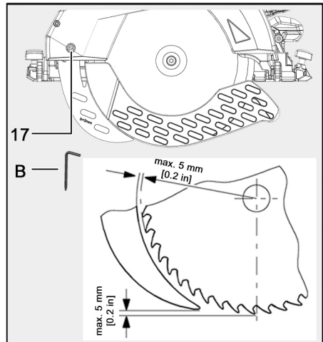
Fig. 13: Distance riving knife to saw blade
