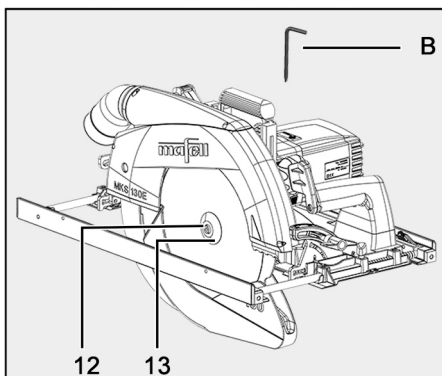
Fig. 5: Removing flange screw and clamping flange
