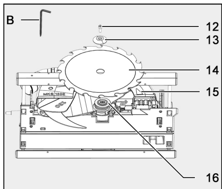
Fig. 8: Replacing the saw blade
