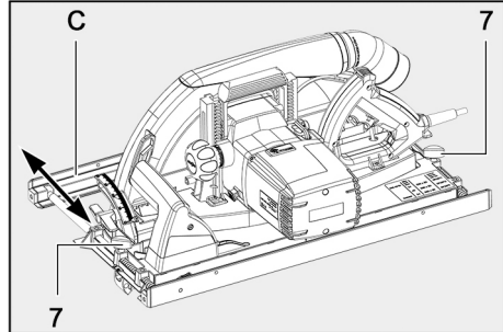
Fig. 16: Adjusting the parallel guide fence
