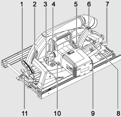
Fig. 2: MKS 130 Ec adjustment elements
