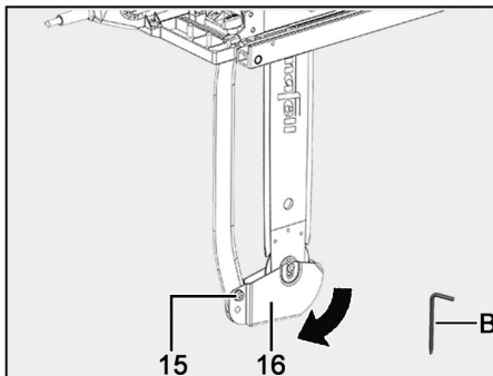
Fig. 6: Opening the guard sheet at the guide bar
