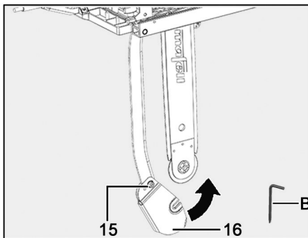
Fig. 11: Closing the guard sheet at the guide bar
