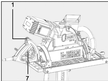
Fig. 32: Switching the machine on
