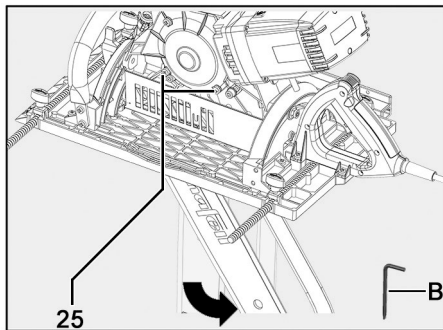
Fig. 36: Swiveling the guide bar to the rear
