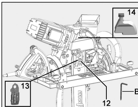
Fig. 24: Inserting intermediate cover and oil tank
