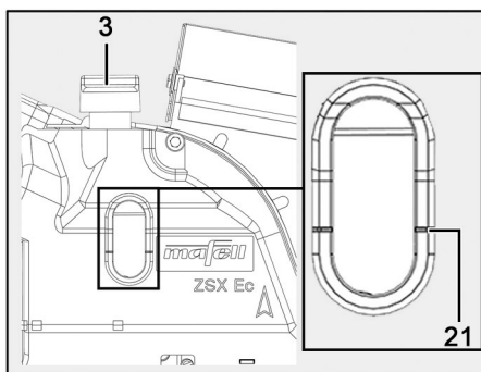
Fig. 19: Oil level in the lubricating oil tank
