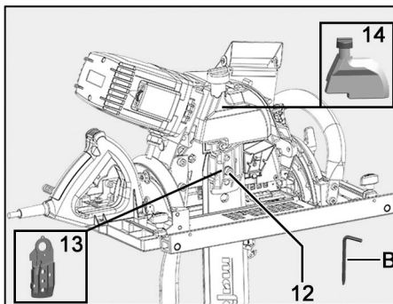
Fig. 5: Removing intermediate cover and oil tank
