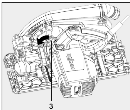
Fig. 8: Closing the guard
