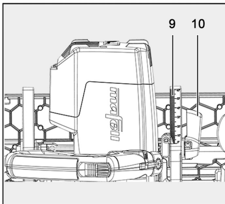
Fig. 15: Setting the saw unit for bevel cuts
