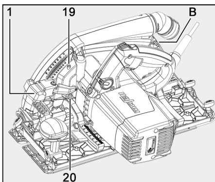
Fig. 18: Resetting the cutting depth
