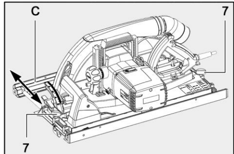
Fig. 19: Adjusting the parallel guide fence
