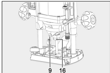
Fig. 10: Unclamping the milling tool
