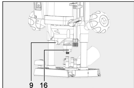
Fig. 8: Removing the adapter
