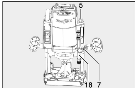
Fig. 18: Adjusting the milling depth using the scale
