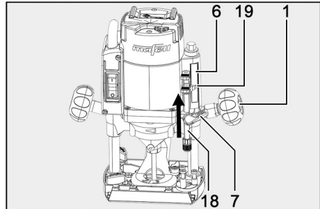
Fig. 17: Adjusting the depth stop
