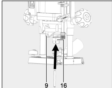
Fig. 9: Clamping the milling tool
