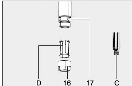
Fig. 7: Installing the adapter
