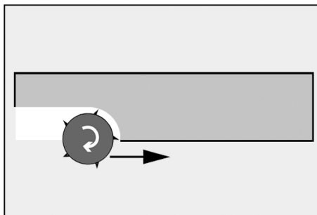
Fig. 20: Climb cutting
