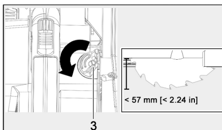
Fig. 27: Deactivating the pre-scoring function
