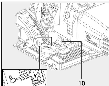
Fig. 18: Setting the saw unit to -1°
