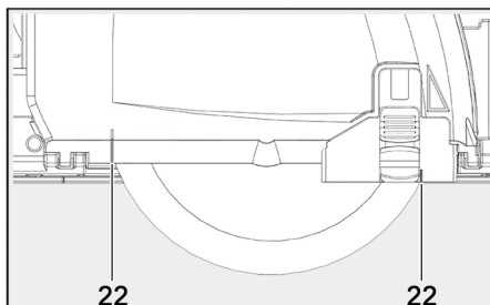
Fig. 20: Plunge cutting
