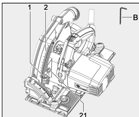
Fig. 16: Setting the cutting depth
