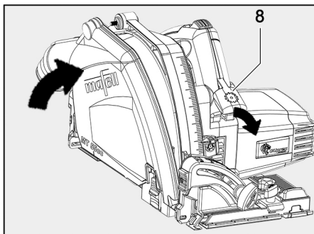
Fig. 11: Closing the guard cover
