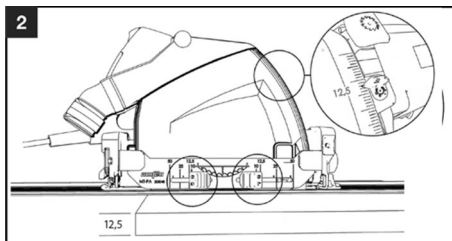
Fig. 29: Setting the cutting depth
