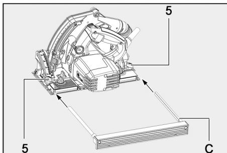
Fig. 22: Installing the parallel guide fence
