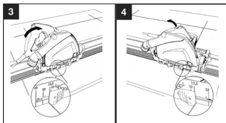
Fig. 30: Setting the position indicator to the cutting depth
