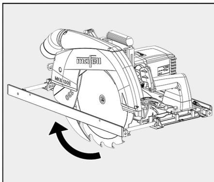
Fig. 9: Opening the guard
