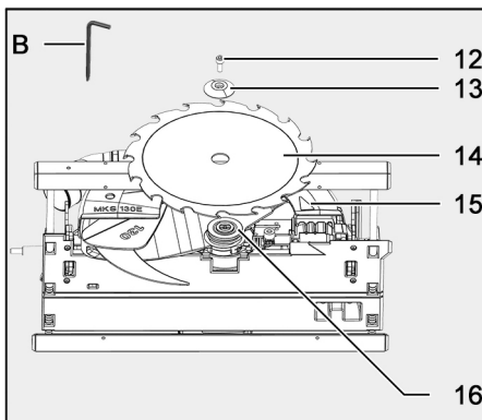
Fig. 11: Replacing the saw blade
