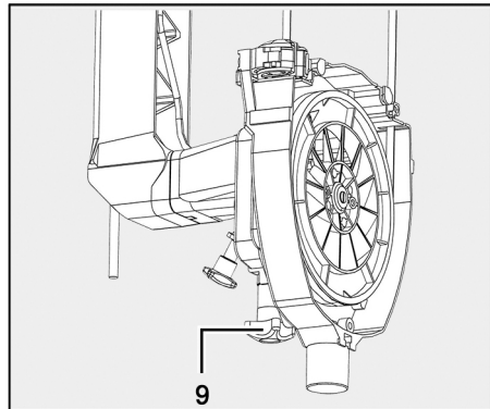
Fig. 5: Releasing the band tension
