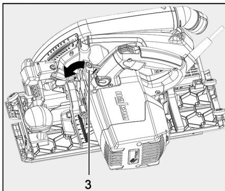
Fig. 8: Unlocking the operating lever
