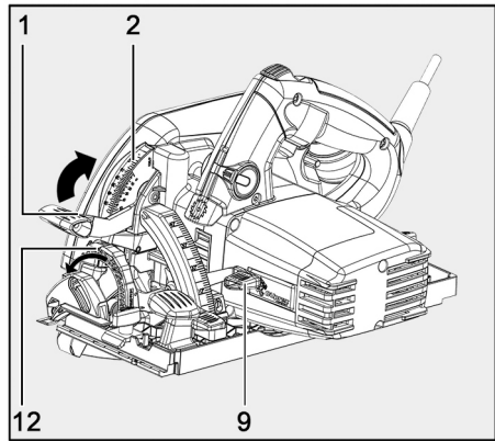
Fig. 16: Plunge cutting
