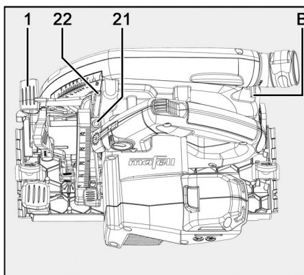
Fig. 18: Resetting the cutting depth
