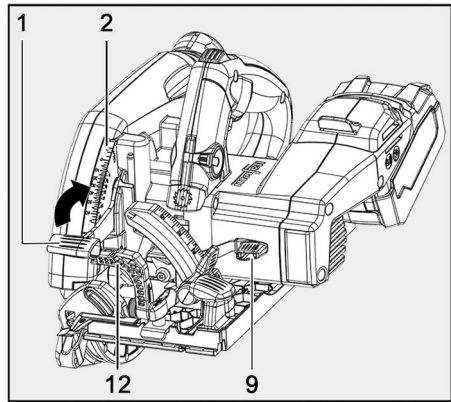
Fig. 19: Plunge cutting
