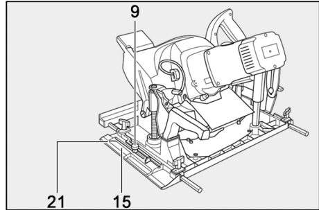
Fig. 13: Setting the marking pointer
