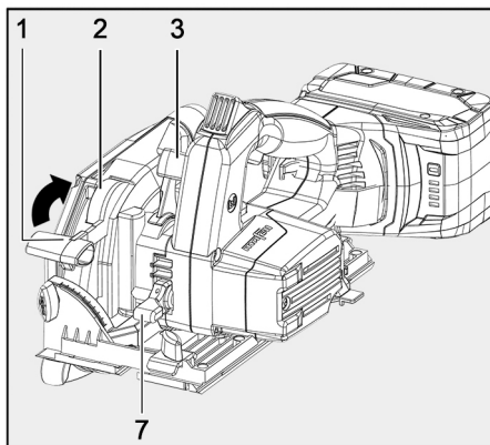
Fig. 15: Plunge cutting
