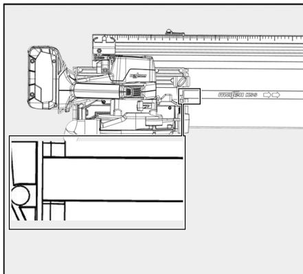
Fig. 22: Placing the machine with the guiding device onto the workpiece
