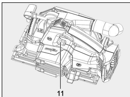
Fig. 6: Actuating the locking pin
