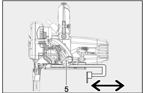
Fig. 22: Adjusting the cutting width via the roller edge guide
