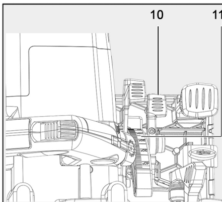
Fig. 16: Setting the saw unit for bevel cuts
